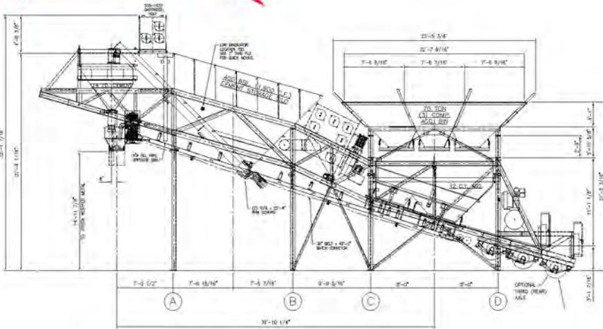
MUSTANG II CONCRETE BATCH PLANT — MAIN ELEVATION FOR 30" BELT BATCH CONVEYOR & 60" DEEP TRUCK HOPPER
