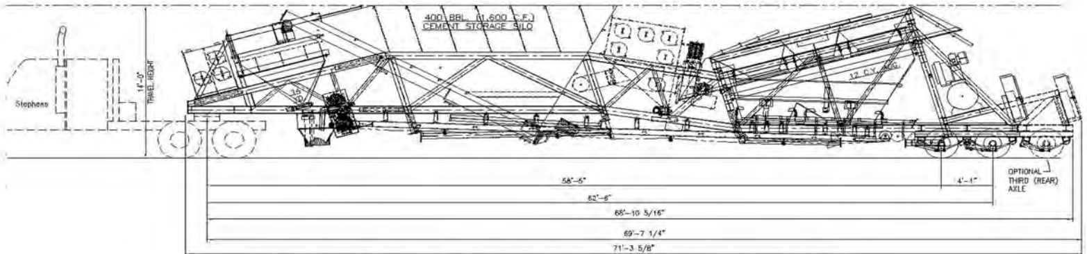
MUSTANG CONCRETE BATCH PLANT — TOWING ARRANGEMENT FOR 30" BELT BATCH CONVEYOR & 60" DEEP TRUCK HOPPER
